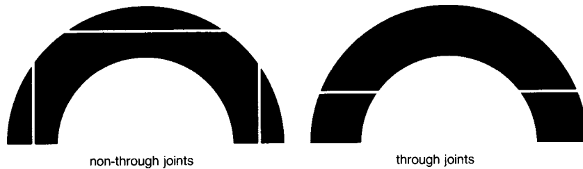
FIG. A3.1 Joint Configuration
